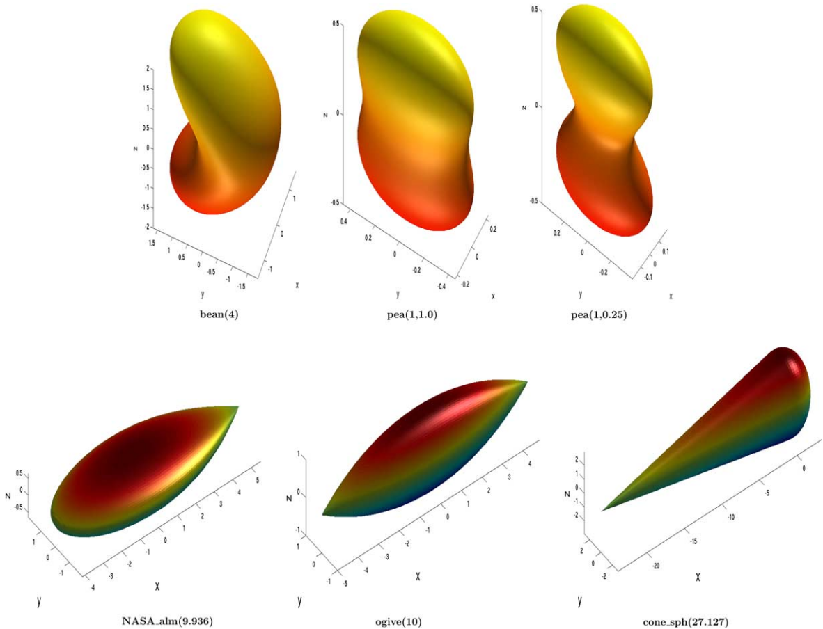
Fig. 1. Some of the obstacles used in our computation.
