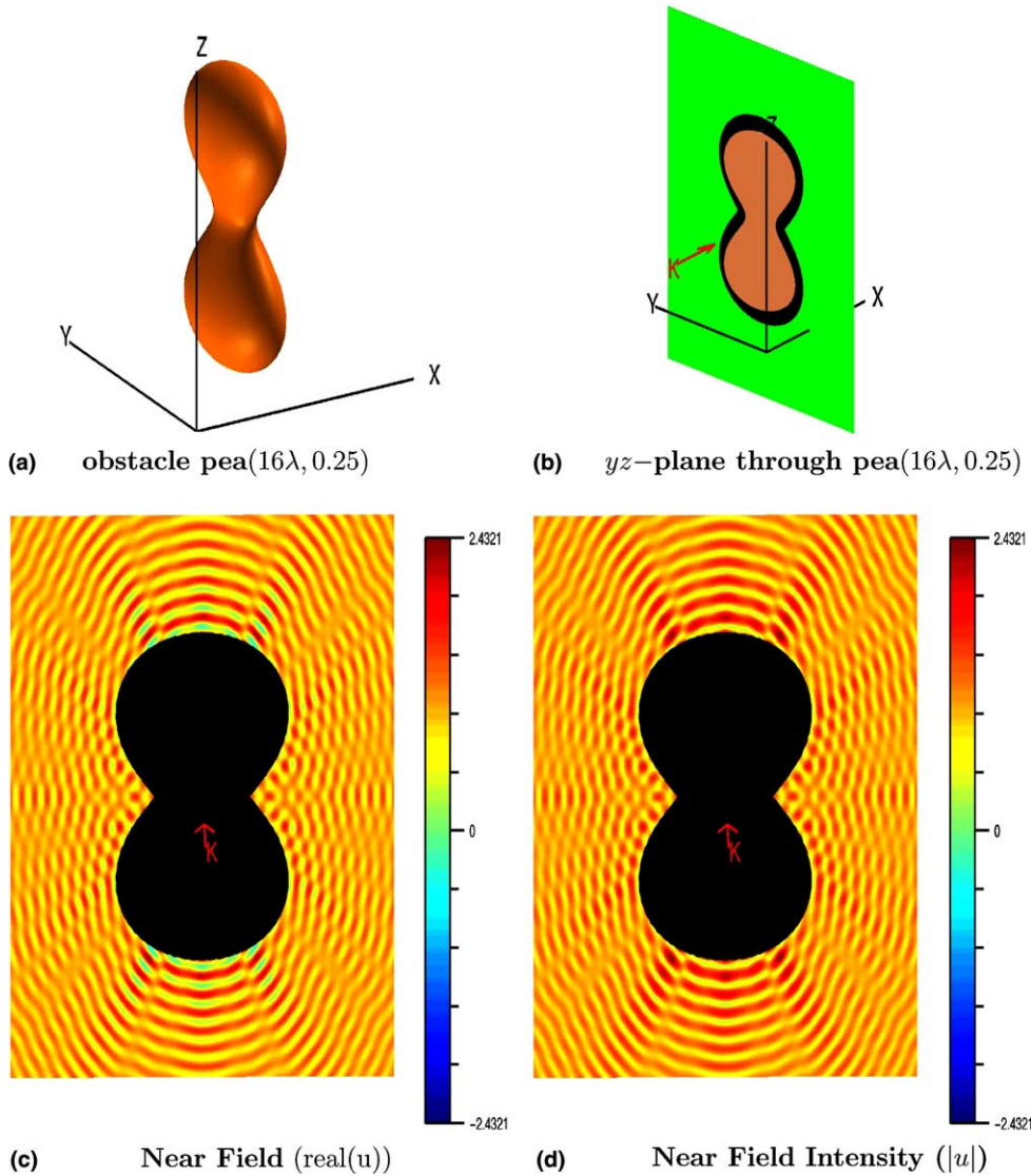
Fig. 2. Visualisation of scattering of a plane wave u^I(\mathbf{x}) = e^{ikx-d} (with k = 100.531 ) propagating in the x -direction (with \hat{\mathbf{d}} = [1, 0, 0] ) by a peanut shaped sound-soft obstacle of size sixteen times the wavelength \lambda = 2\pi/k , on a yz -plane. The scattered field is denoted by u^S and the total field is u = u^I + u^S .
